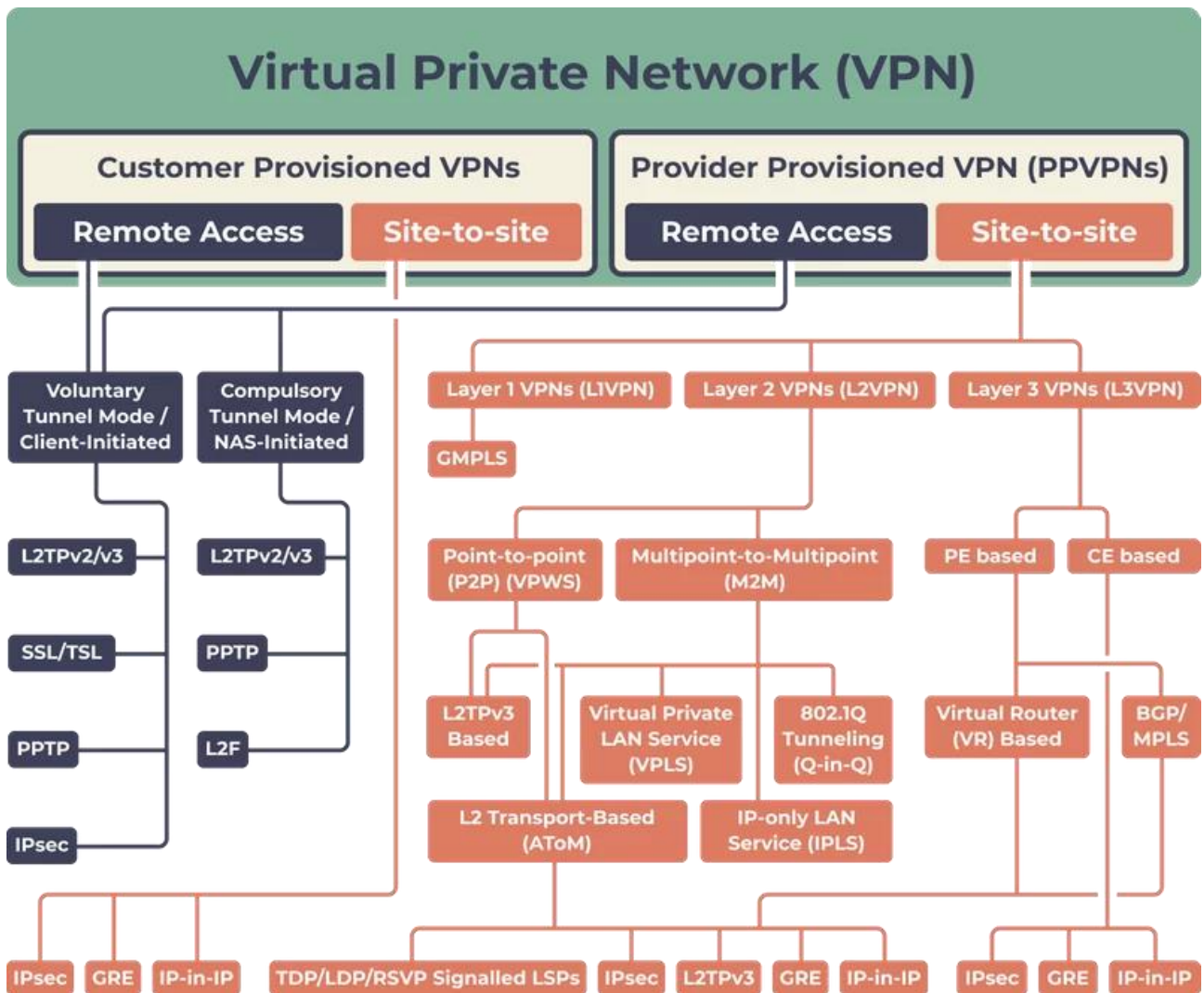
Pic. 2 – Types of VPN
